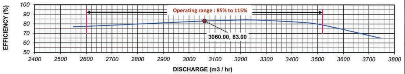
EFFICIENCY VS DISCHARGE
