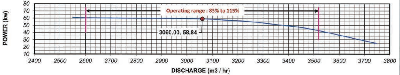
POWER VS DISCHARGE
