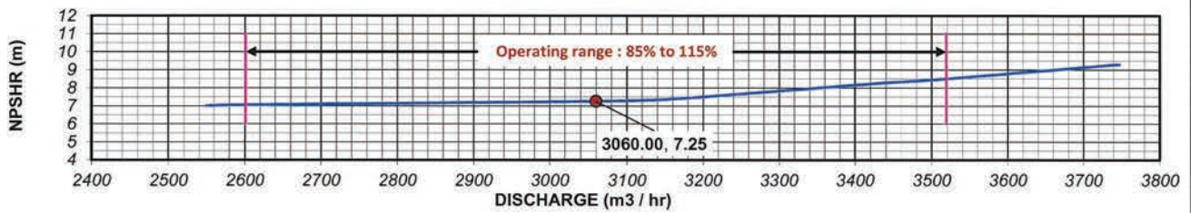
NPSHR VS DISCHARGE
