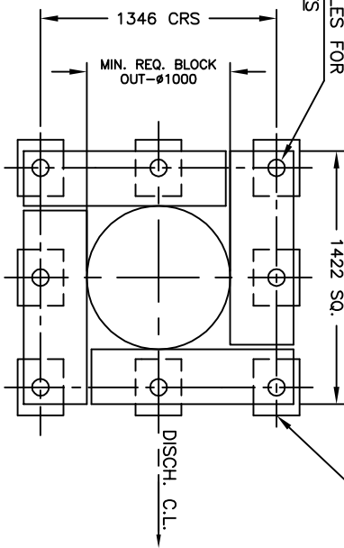
PLAN OF SOLE PLATE AT PUMP FLOOR LEVEL. (+)4.960M ①
