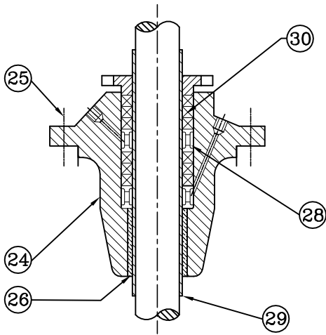
DETAIL OF PACKING BOX A-A
